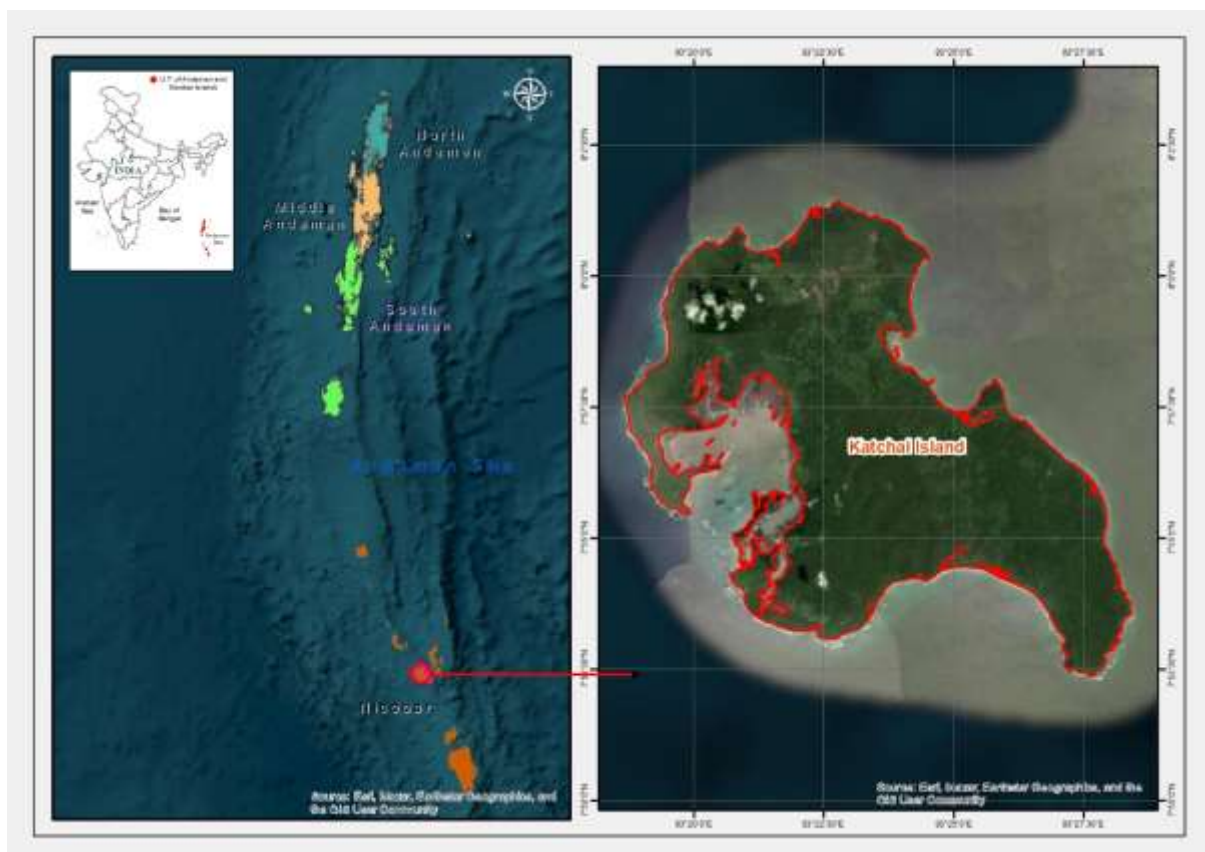
Figure 1. Location map of Katchal Island
