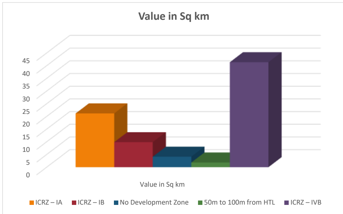
Figure 2. Area statistics of different zone of Katchal Island
