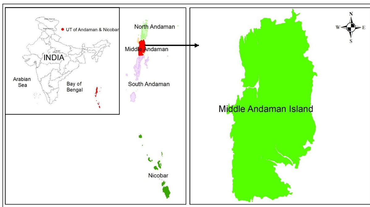
Figure 1. Location map of Middle Andaman Island
